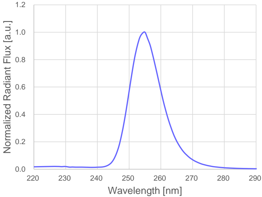
< Spectrum, I_F = 70\text{ mA} >
