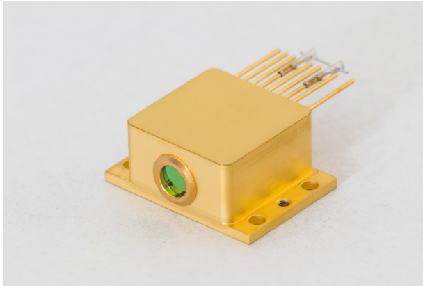
Picture of a HHL with collimated beam output. The lens is inside the housing, protected by a tilted window with AR coating.
